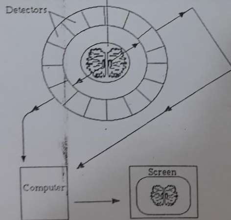
Figure 7.6 The positron-emitting radionuclide ^{11}\text{C} decays to form a positron, which annihilates with an electron. The resulting gamma energy, two photons travelling in opposite directions, can be detected externally by a ring of scintillation detectors placed around the subject in the PET camera.
