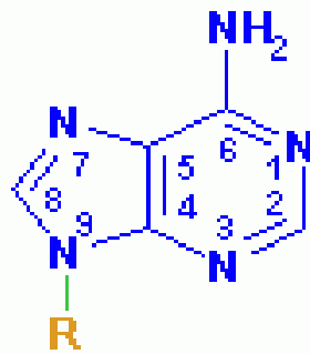
Adenine
