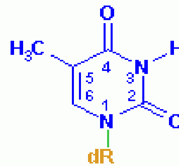
Thymine
