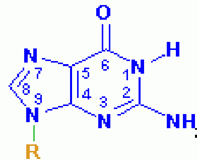
Guanine
