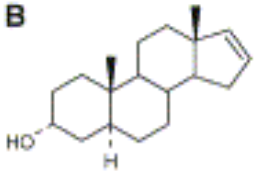
Androst-en-1-ol
