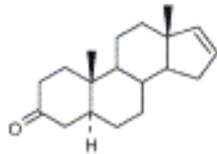
Androst-en-1-one
