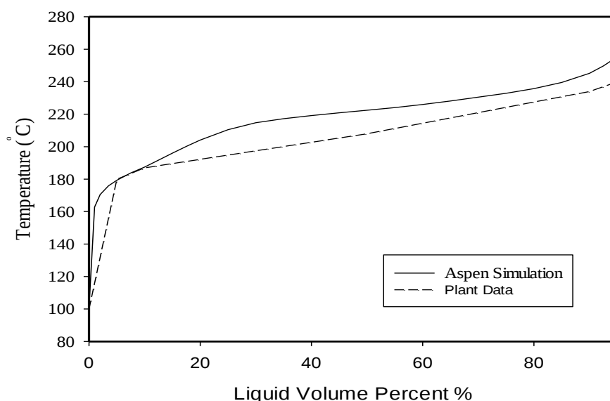
Figure 7: Simulated and plant data ASTM D86 curves of Kerosene.
