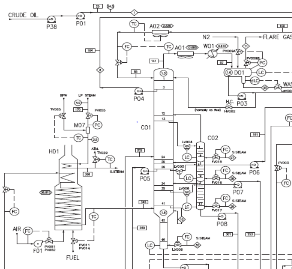
Figure 2: Crude distillation unit in Basrah refinery.
