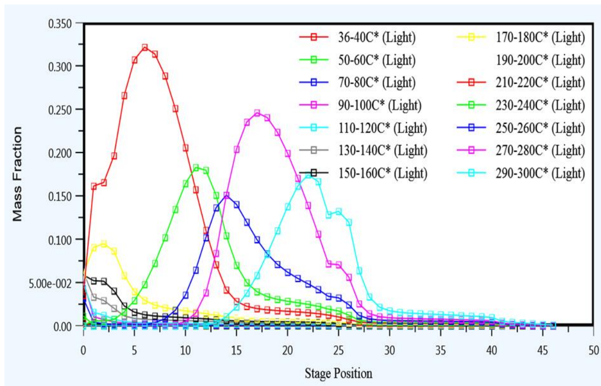
Figure 11: simulated mass fractions for light liquid phase within the column according to boiling points range.
