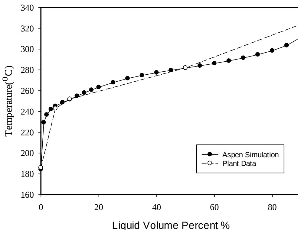
Figure 8: Simulated and plant data ASTM D86 curves of LGO.
