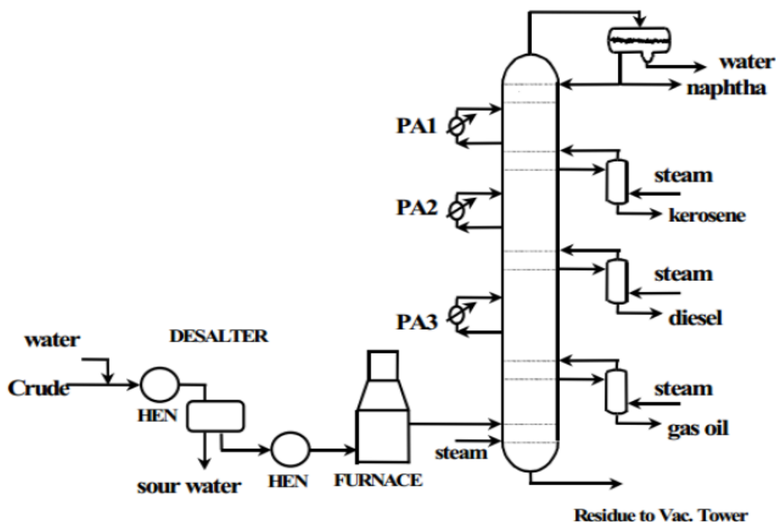
Figure 1: Typical Crude Distillation Unit and Associated Unit Operations.
