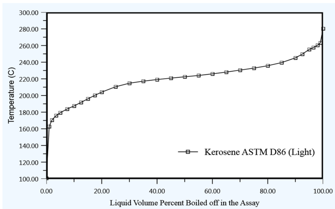
Figure 4: Simulated ASTM D86 curves of Kerosene.
