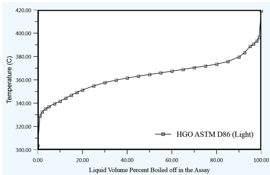
Figure 6: Simulated ASTM D86 curves of HGO.
