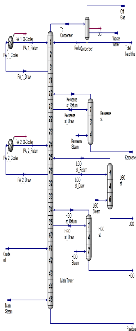
Figure 3: Refinery process flow diagram simulated in Aspen Hysys.
