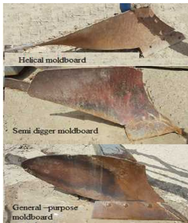
Fig. (1): Moldboard types used in test.
