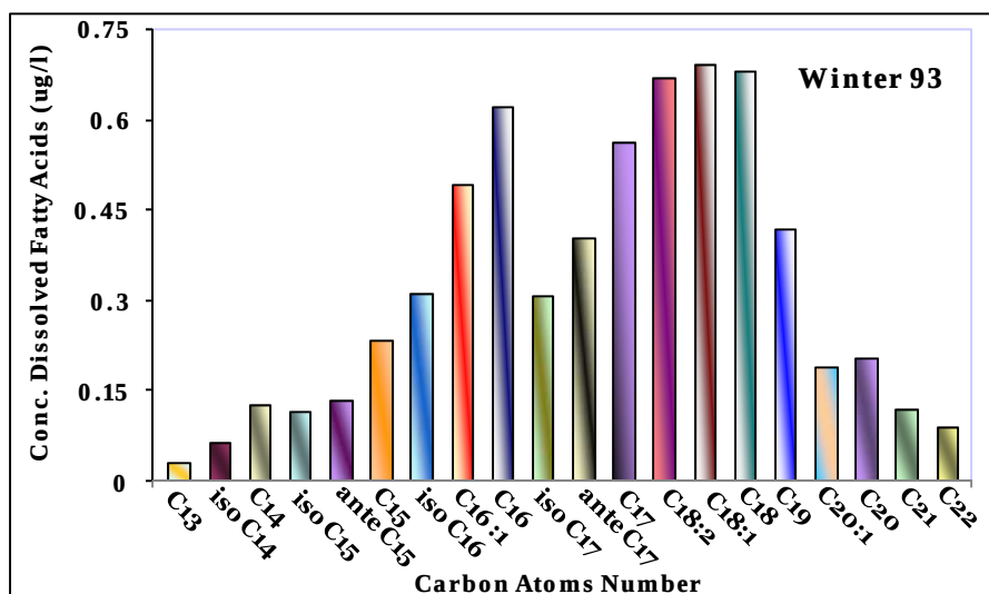
Fig. 4: Mean concentration of dissolved fatty acids ( \mu\text{g/l} ) in the study area during winter 1993.
