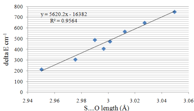
Fig. 2: Correlation between r_{\text{S}\cdots\text{O}} and the enethiol \rightarrow transition state energy barrier
