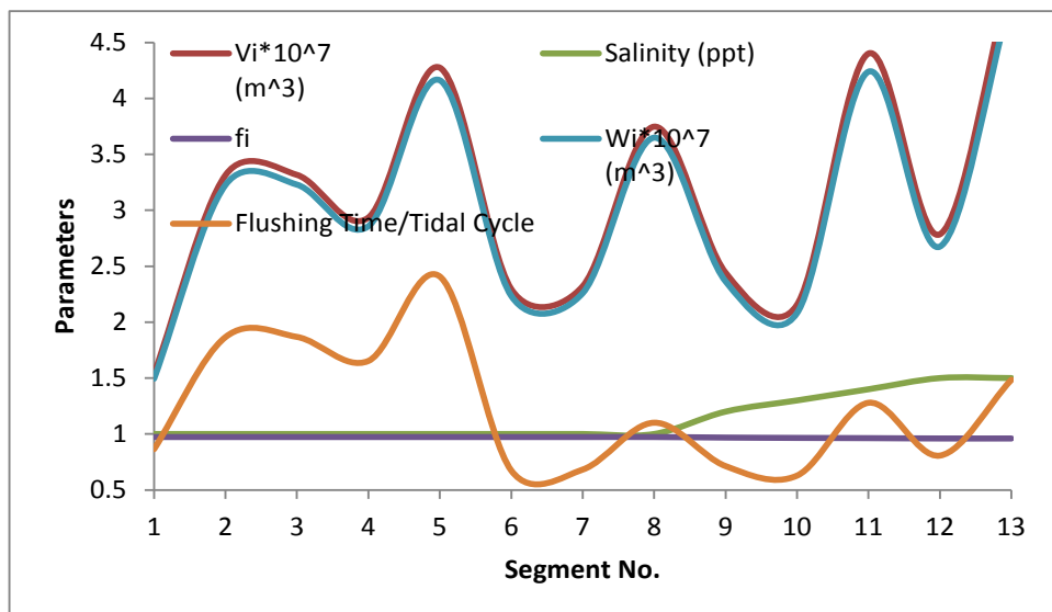
Figure 4. Variation of parameters in first scenario ( Q=800 \text{ m}^3/\text{sec} ).
