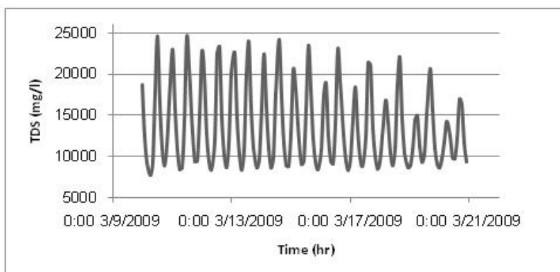
Figure 11. Simulated of TDS at chainage 20000 m in March 2009.
