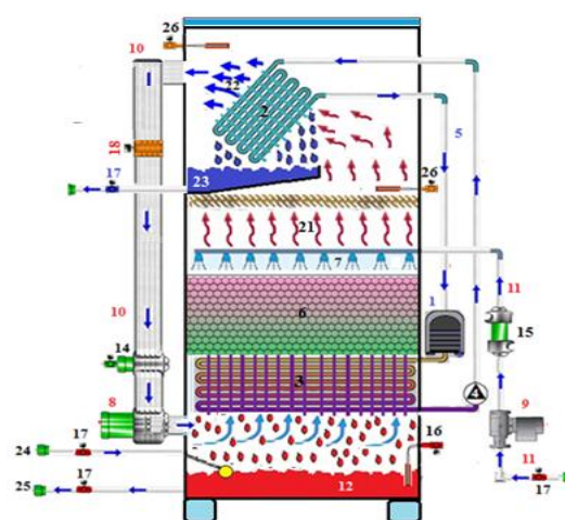
1-Compressor 2-Evaporator 3-Condenser 4-Capillary tube 5-Heat pump pipes 6-Packing material 7-Water distributor 8-Air blower 9-Water pump 10-Air duct 11-Water pipes 12-Feed water tank 13-Distillate collector 14-Rotameter 15-Anemometer 16-Thermometer 17-Water valve 18-Air valve 20-Droplet eliminator 21-Humid air 22-Dry air 23-Fresh water 24-Makeup water 25-Brine 26-Hygrometer.
