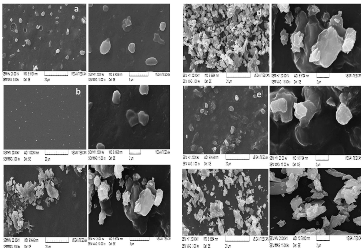
Fig. 1. SEM images of (POT-DBSA/PEO) thin films for all concentrations
