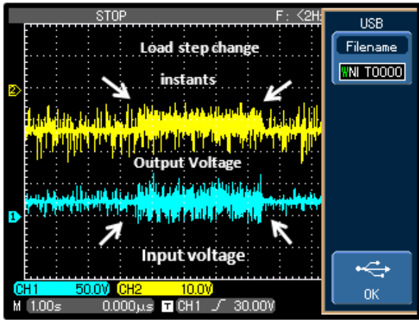
Fig. 8. Input and output voltage profiles, buck mode, two step changes in load resistance 140\Omega to 14\Omega then to 140\Omega , V_{in} = 24V , V_o = -12V , D = 33\%
