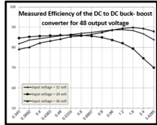
Fig. 10 Measured Efficiency of the DC to DC buck-boost converter for 48 V output voltage
