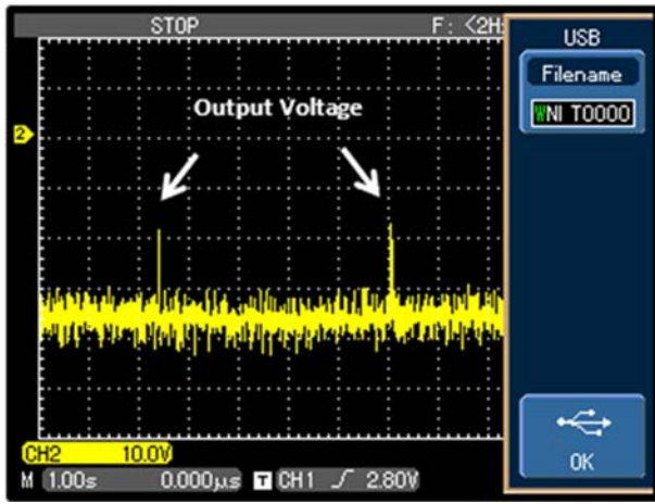
Fig. 7. Output voltage profile, boost mode, two step changes in supply voltage 24V to 28V then to 24V, V_o = -36V , R_L = 140\Omega , D = 60\%
