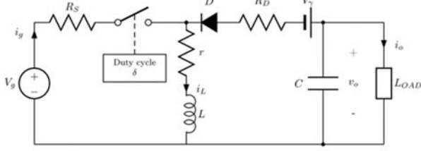
Fig. 2. Buck-boost converter circuit with main non-idealities (losses).
