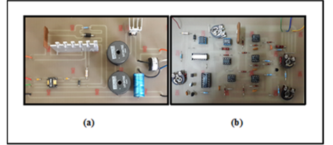
Fig. 5. (a) Experimental setup of the buck-boost converter
