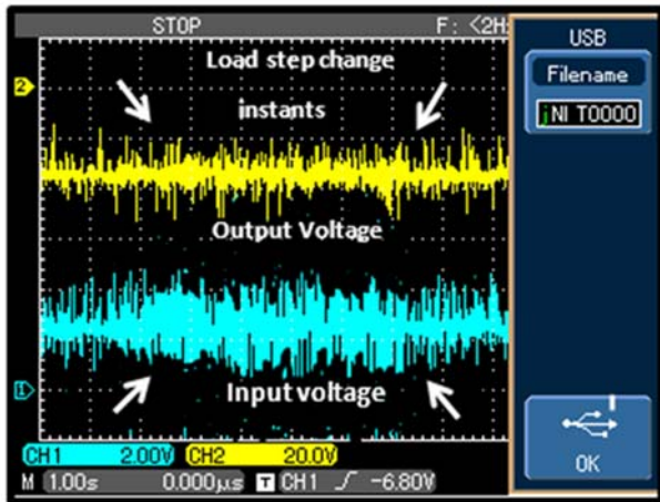
Fig. 9. Input and output voltage profiles, boost mode, two step changes in load resistance 140\Omega to 14\Omega then to 140\Omega , V_{in} = 24V , V_o = -36V , D = 60\%
