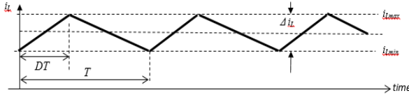
Fig.3. Current through the inductor in the DC-DC buck-boost converter. (Continuous mode of operation CCM) [5]
