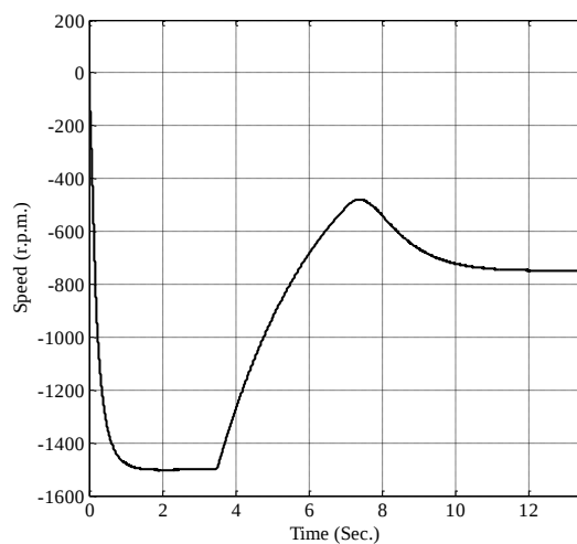
Fig.23 Rotor speed with reference speed is changed
