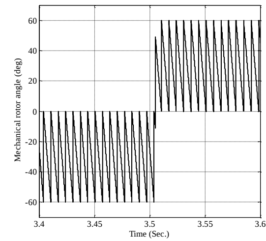
Fig.21 Mechanical rotor position at direction change.
