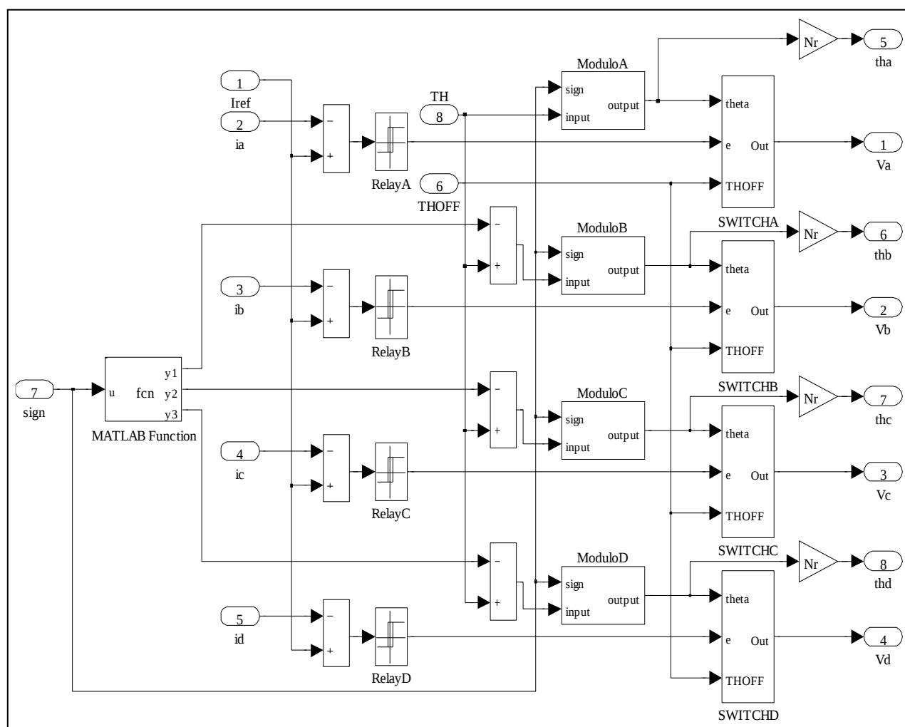
Fig.8 Simulink model of 4 phases 8/6 SRM drive Circuit.
