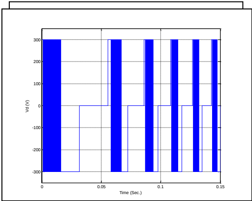
(b)Phase C
