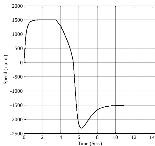
Fig. 25 Mechanical rotor speed when direction is changed
