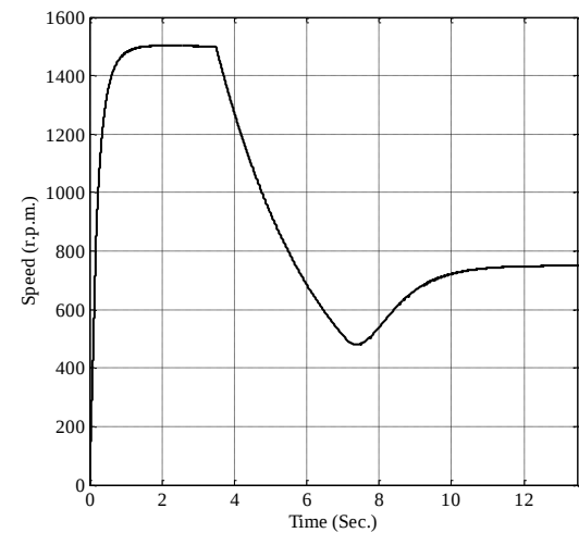
Fig.19 Rotor speed with reference speed step change
