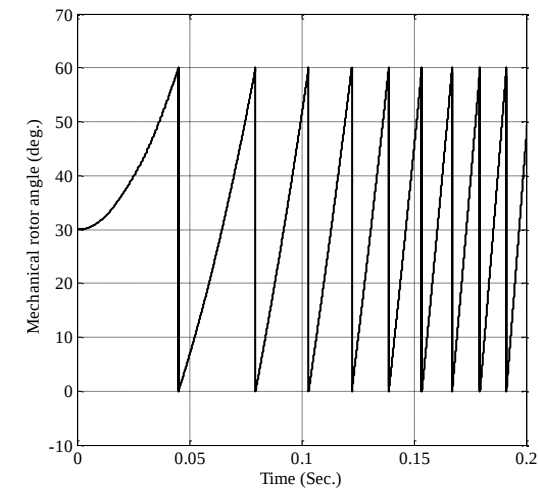
Fig.16 Mechanical rotor position at forward rotation
