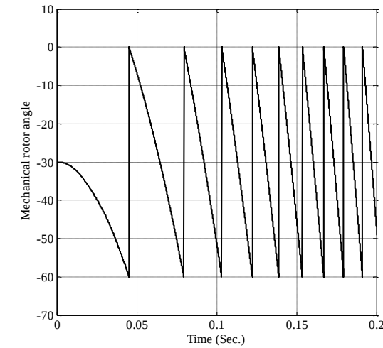
Fig.20 Mechanical rotor position at reverse rotation
