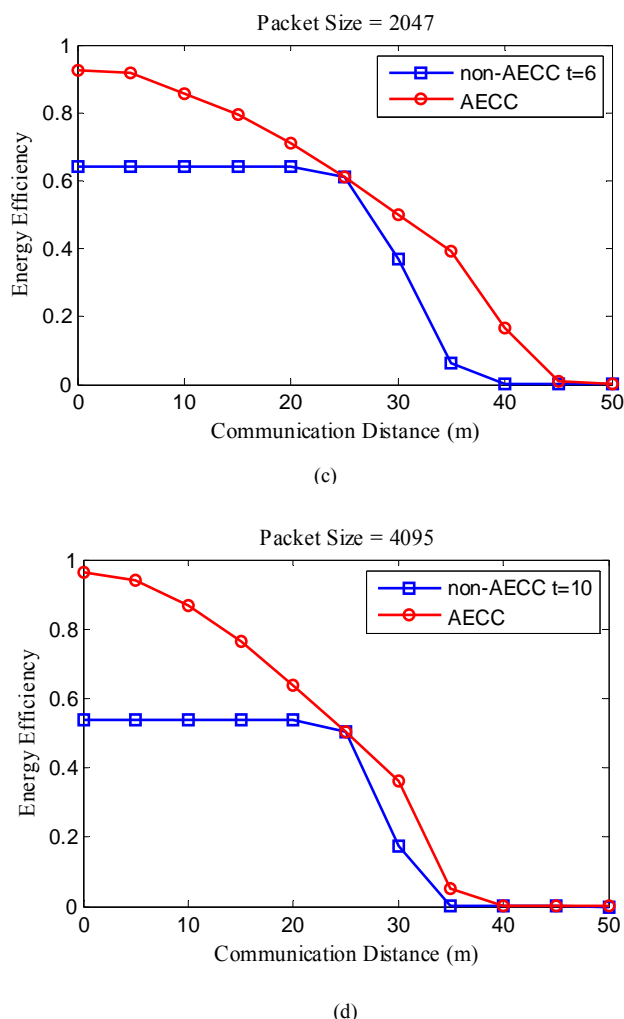
Fig. 4 Energy efficiency of AECC and non-AECC for different packet sizes and communication distance
