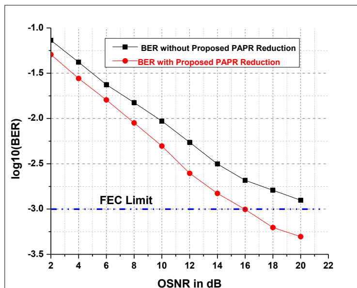
Figure-(8a). BER vs. OSNR.
