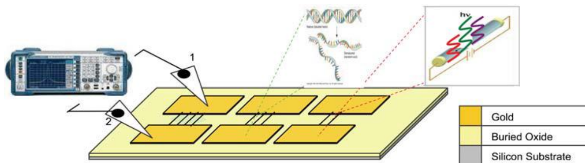
Figure 3. After gold pad formation, measurement of different nanowire pattern using spectrum analyzer semiconductor parameter analyzer are taken (Uda et al., 2008).
