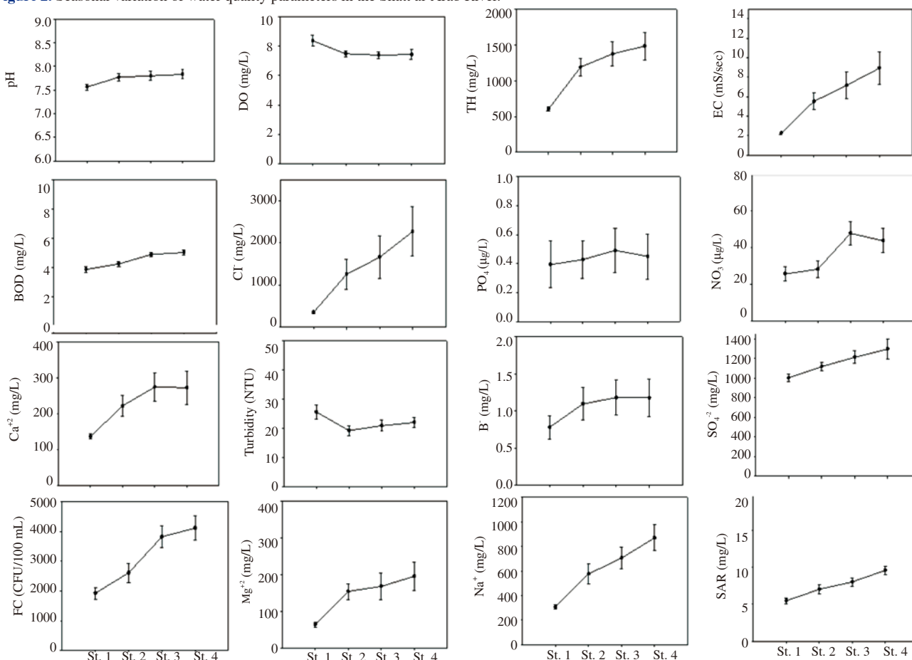
Figure 3. Spatial variation of the four stations along the axis of Shatt al-Arab River.
