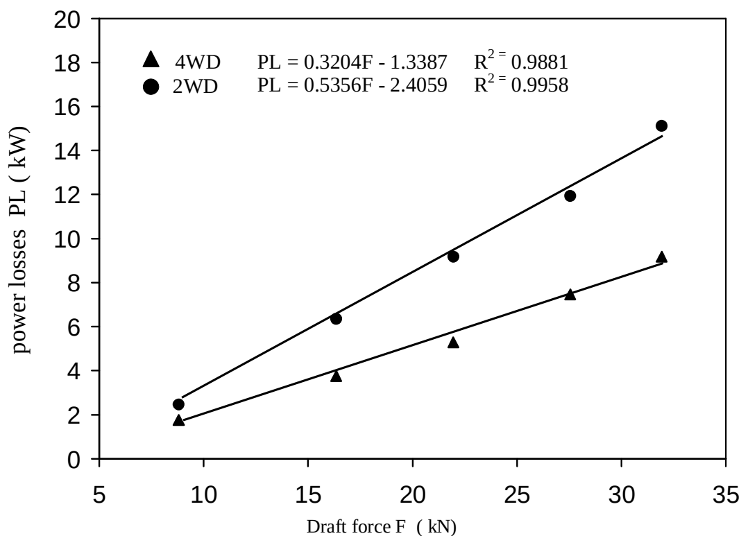
Figure (1) : The relationship between the draft force and the power losses for tractor MF( 2680 )
