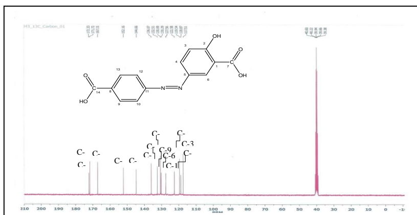
Figure 8: 13 C-NMR spectrum of compound 2c
