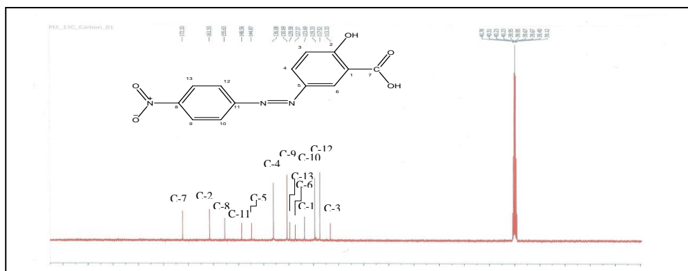
Figure 7: 13 C-NMR spectrum of compound 2b
