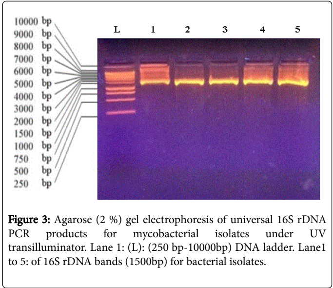
Figure 3: Agarose (2 %) gel electrophoresis of universal 16S rDNA PCR products for mycobacterial isolates under UV transilluminator. Lane 1: (L): (250 bp-10000bp) DNA ladder. Lane1 to 5: of 16S rDNA bands (1500bp) for bacterial isolates.
