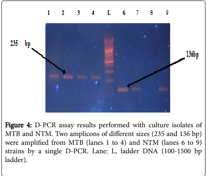
Figure 4: D-PCR assay results performed with culture isolates of MTB and NTM. Two amplicons of different sizes (235 and 136 bp) were amplified from MTB (lanes 1 to 4) and NTM (lanes 6 to 9) strains by a single D-PCR. Lane: L, ladder DNA (100-1500 bp ladder).
