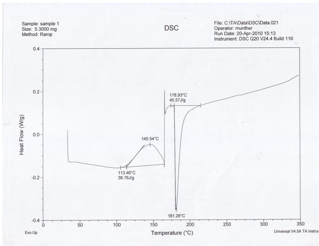
Figure ( 4 ) : DSC thermogram of polyallyloxyvinylsilane
