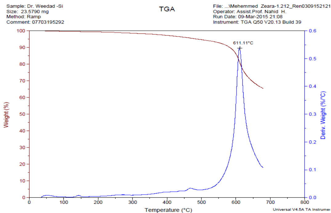
.Figure ( 3 ) : TGA &DTGA Thermograme of polyallyloxyvinyl silane
