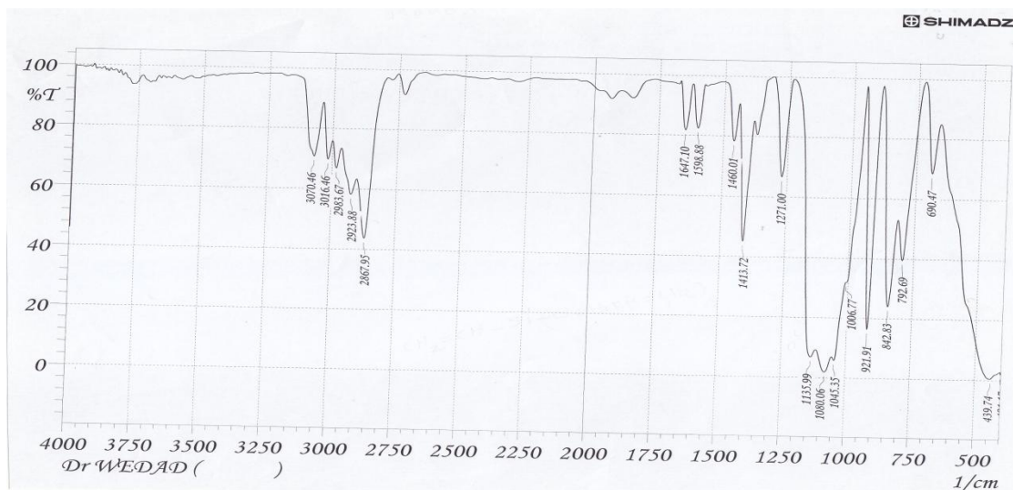
Figure (1) : FTIR spectrum of vinyltriallyloxysilane monomer.
