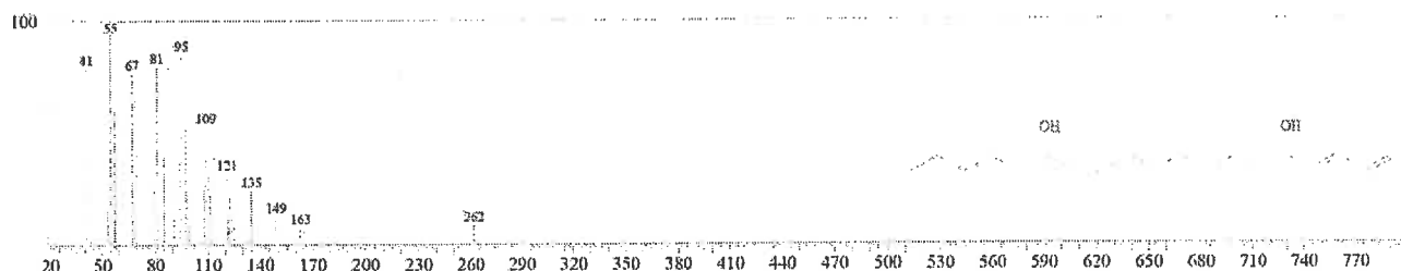
E,E,Z-1,3,12- Nonadecatriene-5,14,-diol.
