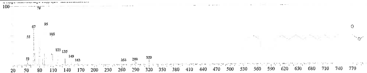
Methyl 11,14,17,-eicosatrienoate
