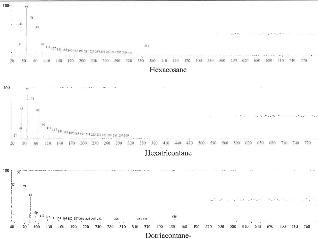
Figure (2): Mass spectra of active chemical compounds separated from lipids of Capparis spinosa L. and characterized by mass spectroscopy.
