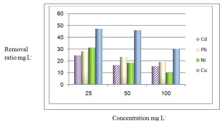
Figure 4. Heavy metal uptake by Bacillus megaterium in different concentration
