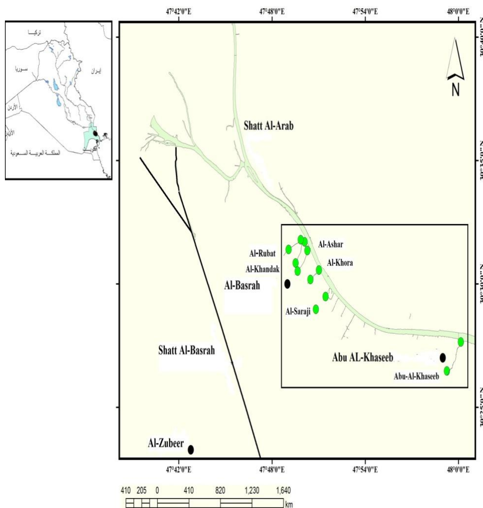
Fig. 1. Location of inner rivers in Basra governorate-Iraq
