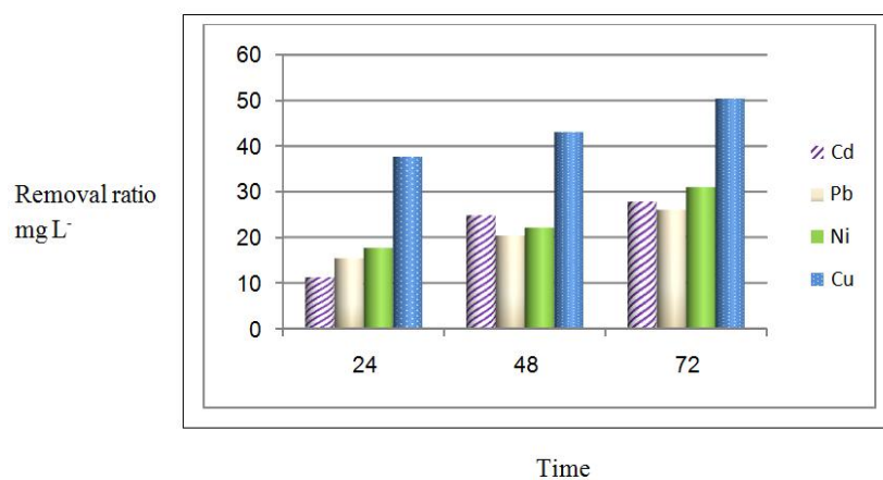
Figure 5. Heavy metal uptake by Bacillus spp. in different time
