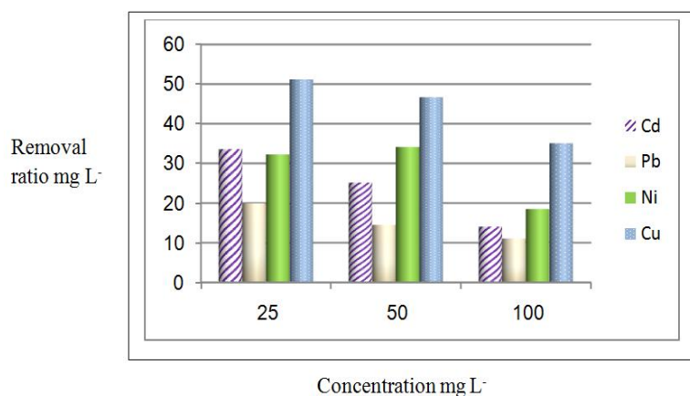
Figure 2. Heavy metal uptake by Bacillus licheniformis in different concentrations
