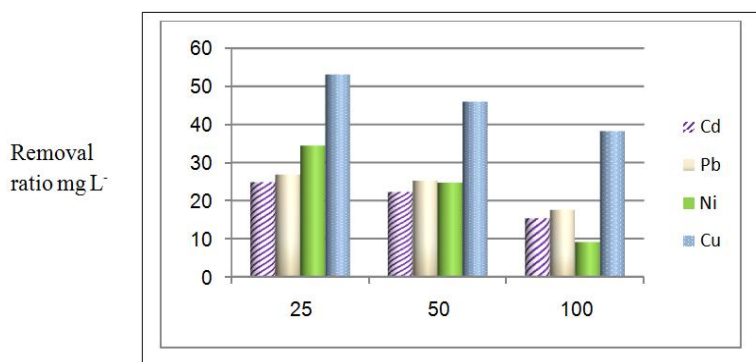
Figure 3. Heavy metal uptake by Bacillus badius in different concentrations
