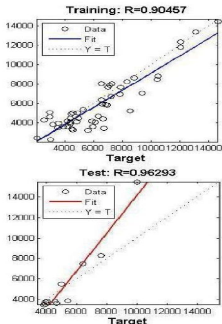
Fig.2 Monthly electrical conductivity (EC) estimates by Neural Networks versus the corresponding monthly measured values at study area, for the training and the testing sets
