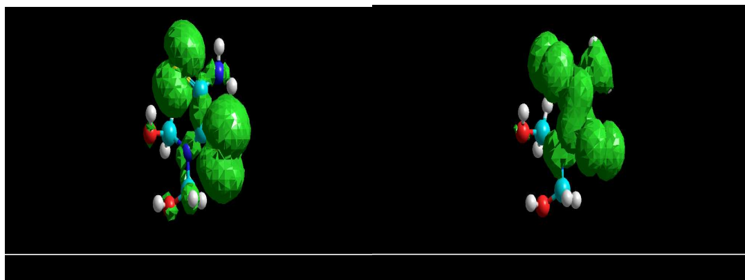
(b)HOMO interaction.
