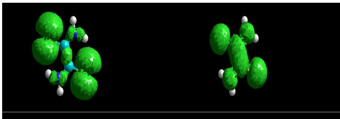
(b)HOMO interaction.
