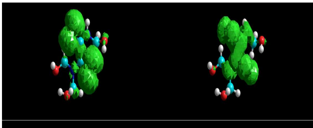
(b)HOMO interaction.
