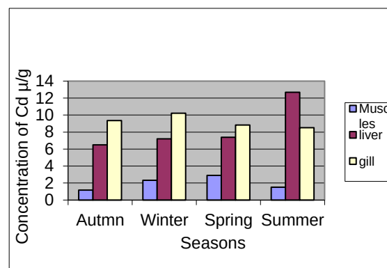
Figure 6. Concentration of Cadmium ( \mu\text{g/gm} ) dry weight in the Muscles, Liver, and gill tissues, during four seasons.
