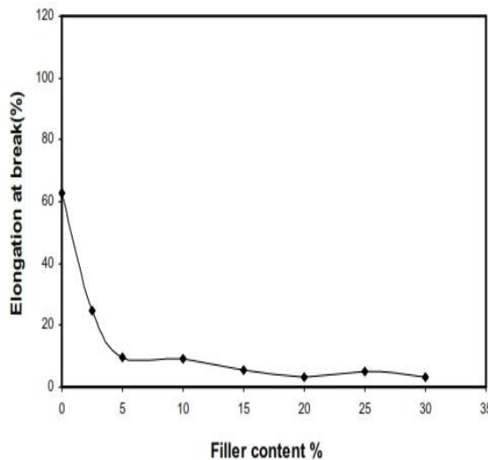
Figure (6) Elongation at break and powder of Alum - HDPE composites.
