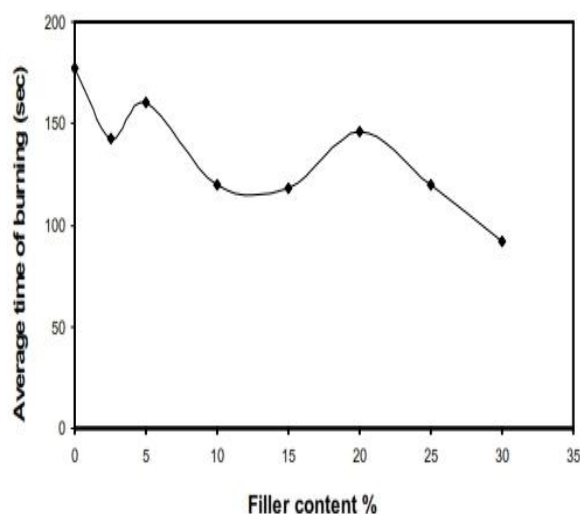
Figure (9) relation between the ATB and Alum powder- HDPE composites.
