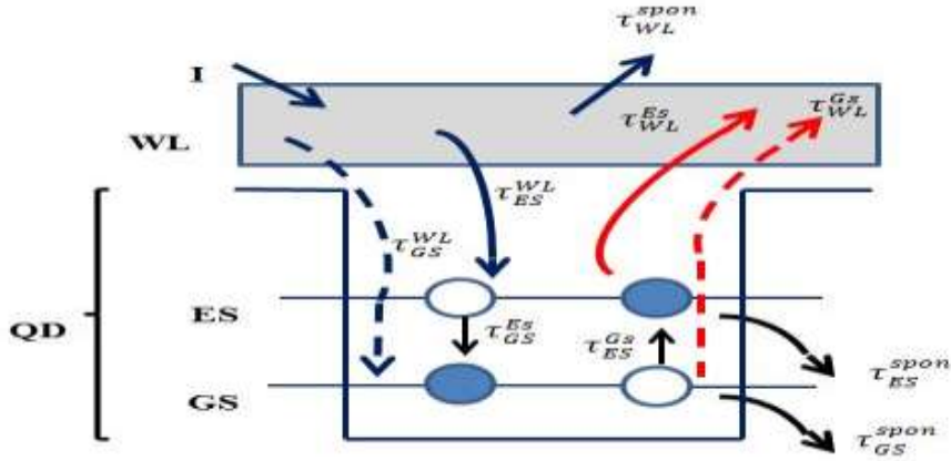
Fig. (1): Carrier dynamics representation with direct (dashed line) relaxation channel schematically in a quantum dot laser.
