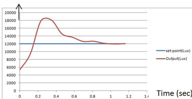
Fig. 16 the system response of light system control.
