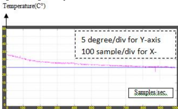
Fig. 14 Set-Point is 25^{\circ} and the initial value is 35^{\circ}
