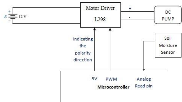
Fig. 3 Pump's Control Circuit.
