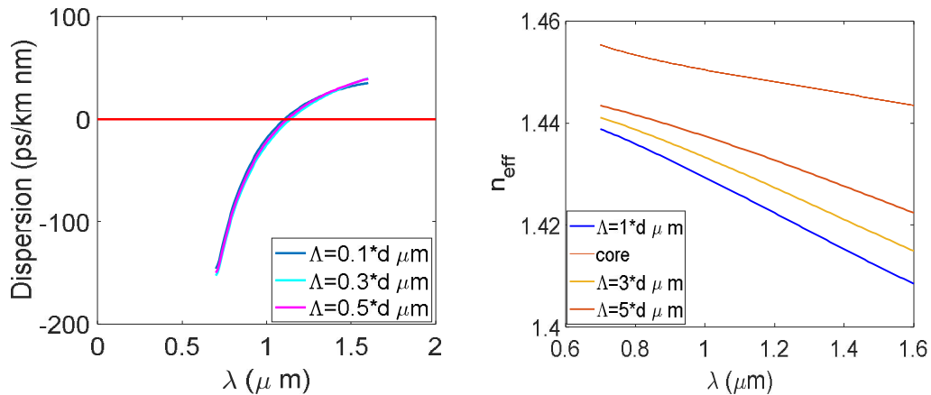
Figure (1): The dispersion curves (left), and n_{\text{eff}} (right), changes with wavelength at d=0.3 \mu\text{m} , N=5 .
