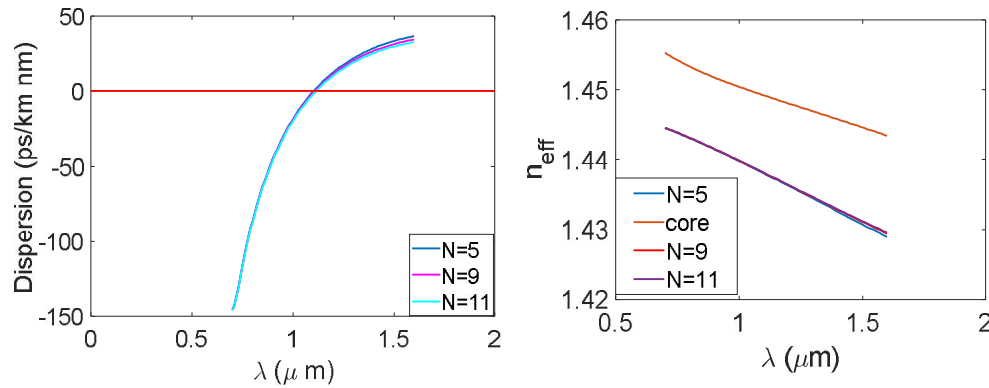
Figure (3): The dispersion curve and n_{\text{eff}} for different values of hole number.
