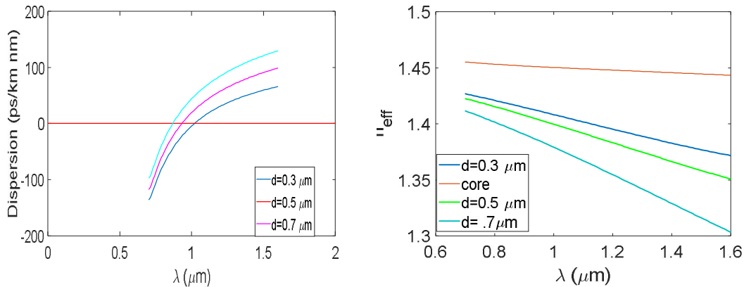
Figure (2): The dispersion curve and n_{\text{eff}} for different values of hole diameter.
