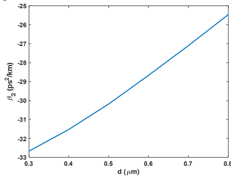
Figure (4): The relation between \beta_2 and the hole diameter, d .
