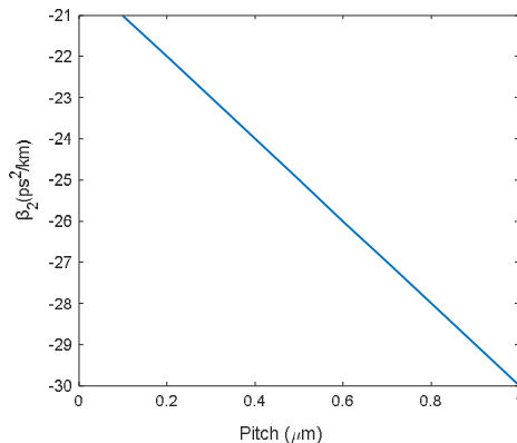
Figure (5): The relation between \beta_2 and the pitch, \Lambda .
