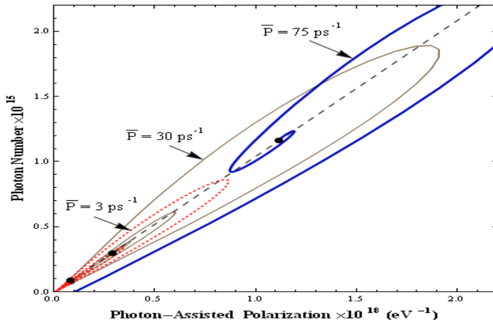
Figure 5: The Attractor between Photon-Assisted Polarization and Photon Number of InGaAs/GaAs QDL at 1.3 \mu\text{m} Wave-Length for Different Values of Pump Pulse Area ( \bar{P} ): 3ps -1 (Dotted Curve), 30ps -1 (Thin Curve), and 75ps -1 (Thick Curve)
