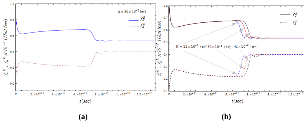
Fig. 4 a) variations of the carrier density with time at the ground level are connected curve for f_e^E , and the dashed curve for f_h^E with k = 30 \times 10^{-6} eV. (b) The time variation of the different values of k = (12, 30, 42) \times 10^{-6} eV.
