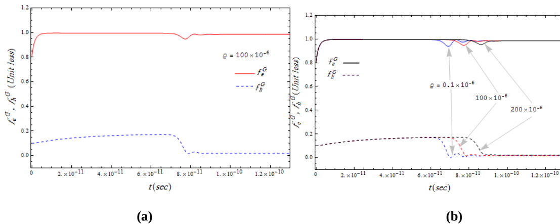
Fig. 1 (a) variations of the carrier density with time at the ground level are connected curve for f_e^G , and the dashed curve for f_h^G with \varrho = 100 \times 10^{-6} . (b) The time variation of the different values of \varrho = (0.1, 100, 200) \times 10^{-6} . Other parameters values as listed in Table (1).
