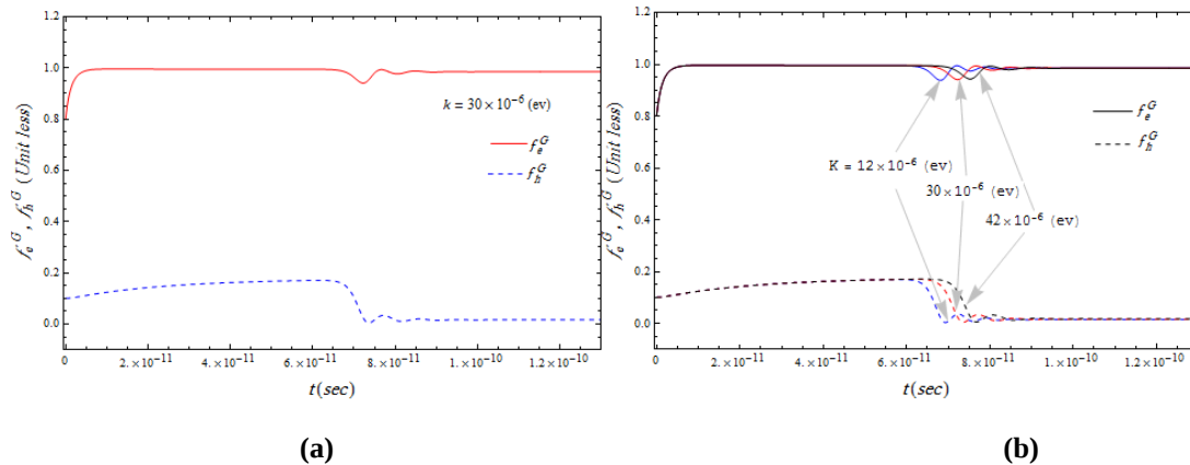
Fig. 3 (a) variations of the carrier density with time at the ground level are connected curve for f_e^G , and the dashed curve for f_h^G with k = 30 \times 10^{-6} eV. (b) The time variation of the different values of k = (12, 30, 42) \times 10^{-6} eV.
