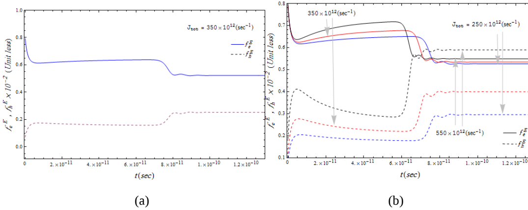
Fig. 8 a) variations of the carrier density with time at the ground level are connected curve for f_e^E , and the dashed curve for f_h^E with J_{tot} = 350 \times 10^{12} \text{ (sec}^{-1}\text{)} . (b) The time variation of the different values of J_{tot} = (250, 350, 550) \times 10^{12} \text{ (sec}^{-1}\text{)} .
