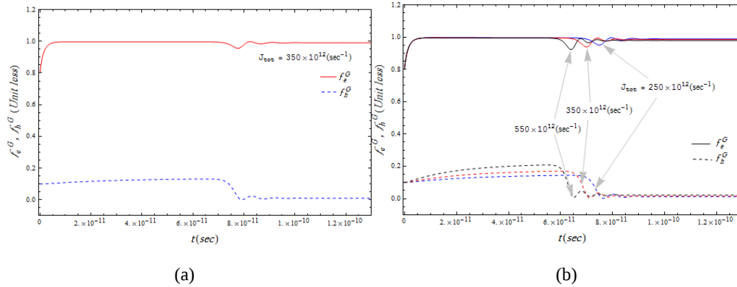
Fig. 7 (a) variations of the carrier density with time at the ground level are connected curve for f_e^G , and the dashed curve for f_h^G with J_{tot} = 350 \times 10^{12} \text{ (sec}^{-1}\text{)} . (b) The time variation of the different values of J_{tot} = (250, 350, 550) \times 10^{12} \text{ (sec}^{-1}\text{)}
