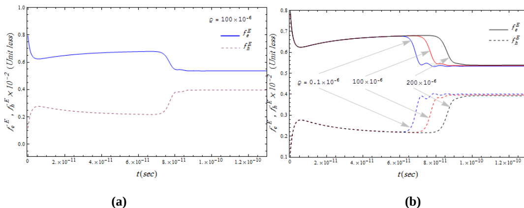
Fig. 2 a) variations of the carrier density with time at the ground level are connected curve for f_e^E , and the dashed curve for f_h^E with \varrho = 100 \times 10^{-6} . (b) The time variation of the different values of \varrho = (0.1, 100, 200) \times 10^{-6} .
