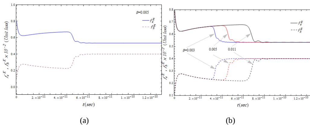
Fig. 6 a) variations of the carrier density with time at the ground level are connected curve for f_e^E , and the dashed curve for f_h^E with \beta = 0.005 . (b) The time variation of the different values of \beta = (0.003, 0.005, 0.011) .
