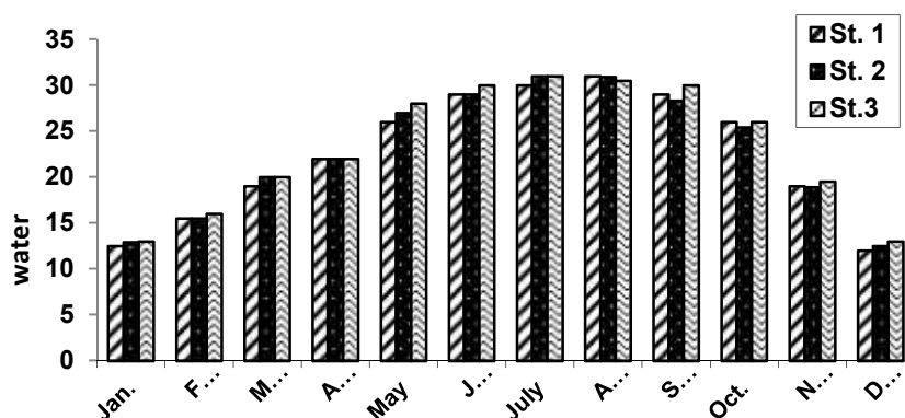
Fig. (2): Monthly variation in water temperature (°C) at the studied stations during the period from January to December 2015.
